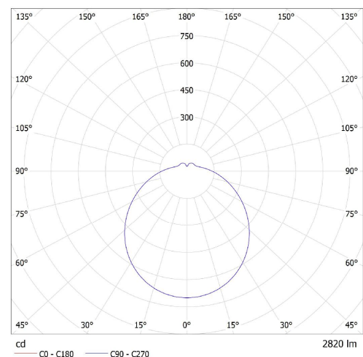
Lucis S44.L16.CA4 CHARON PMMA LED / LDC (Polar)
